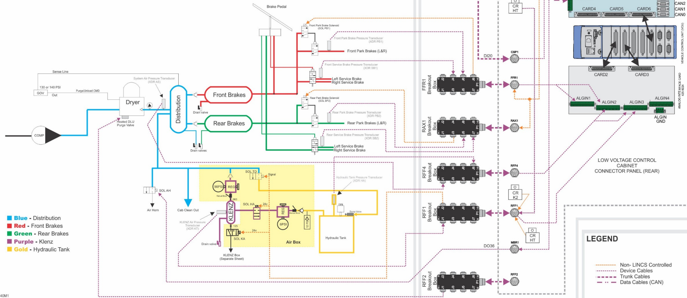
Figure 8. Complete air system
