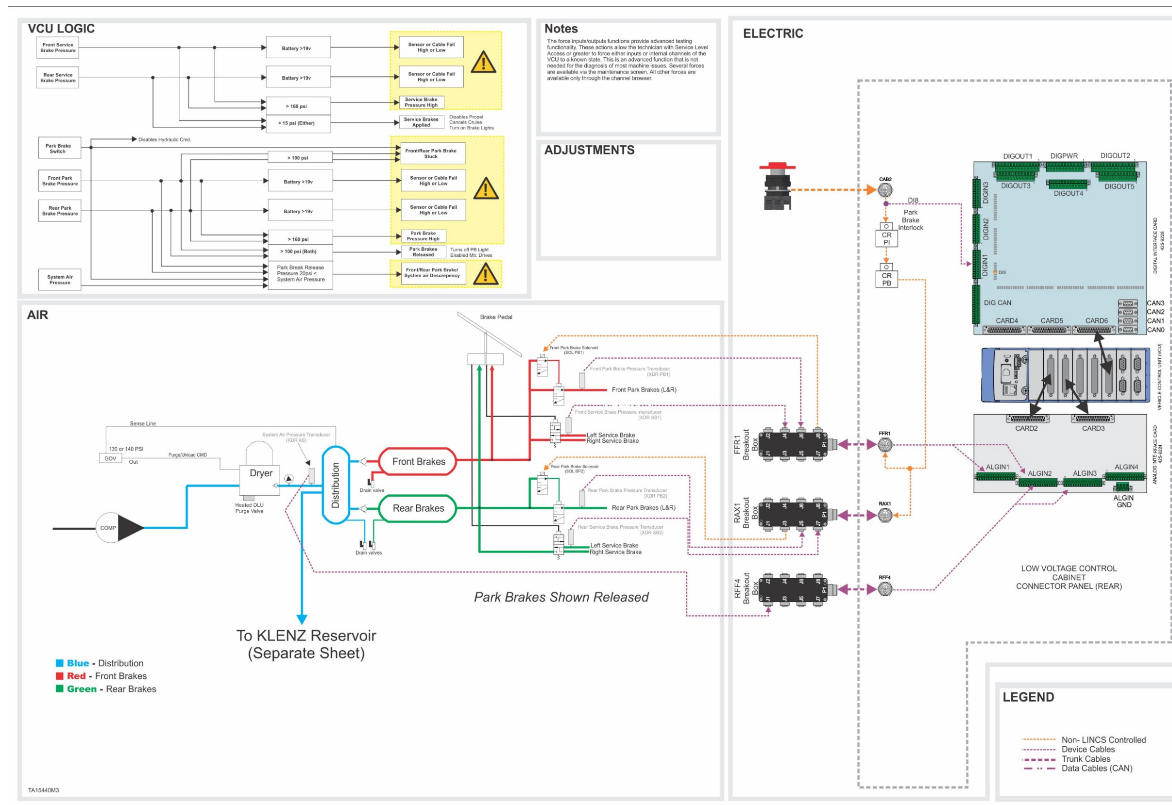
Figure 10. Brake system
